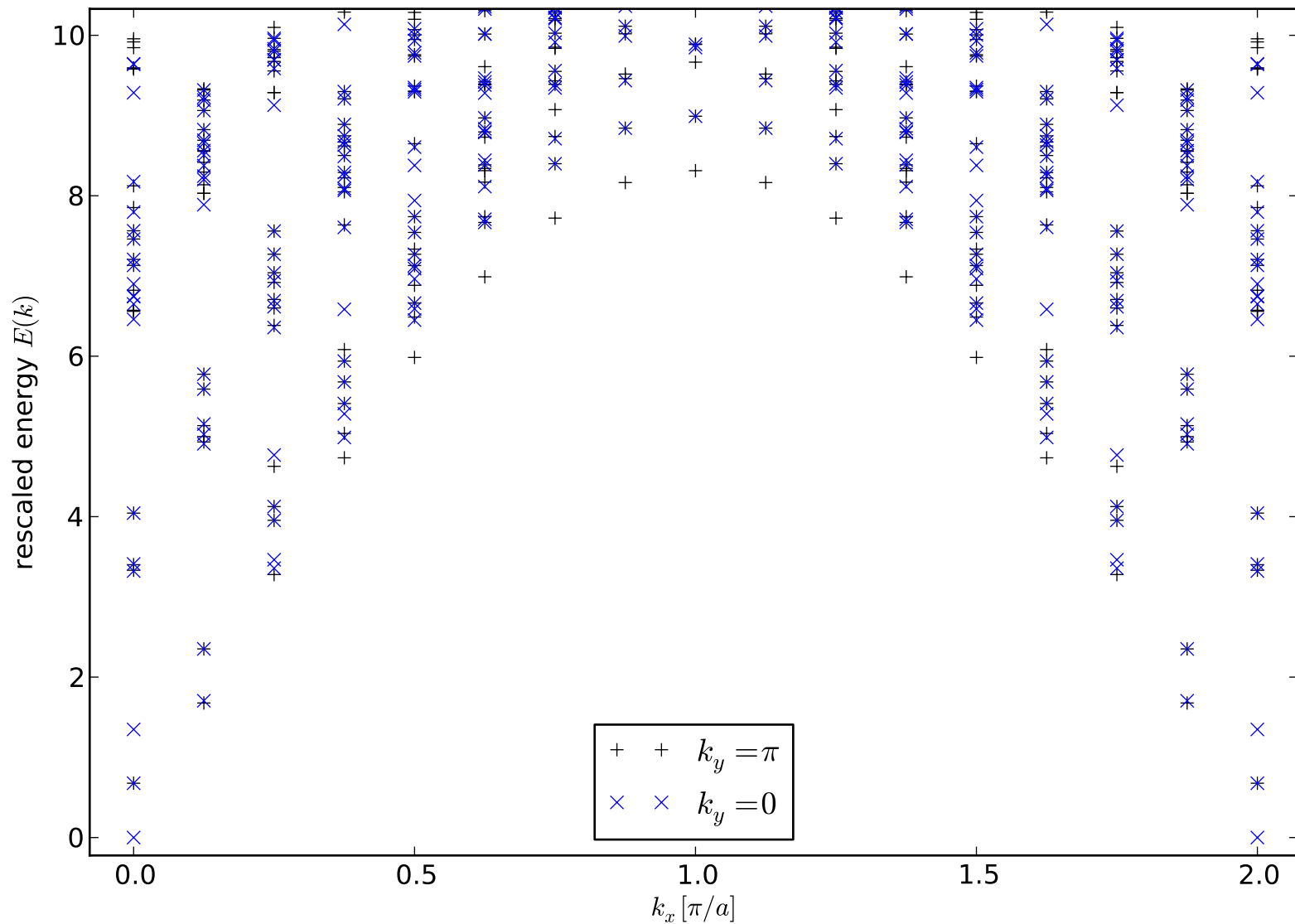
Spectrum: Galois conjugate on the ladder (effective model \theta \rightarrow \frac{3\pi}{2} , L=16)
