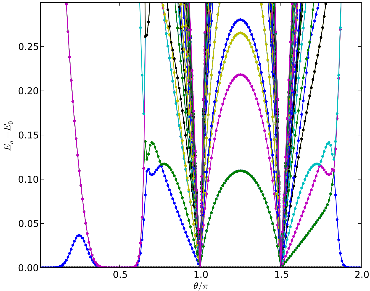
Spectrum of Galois conjugate on 8-rung ladder
