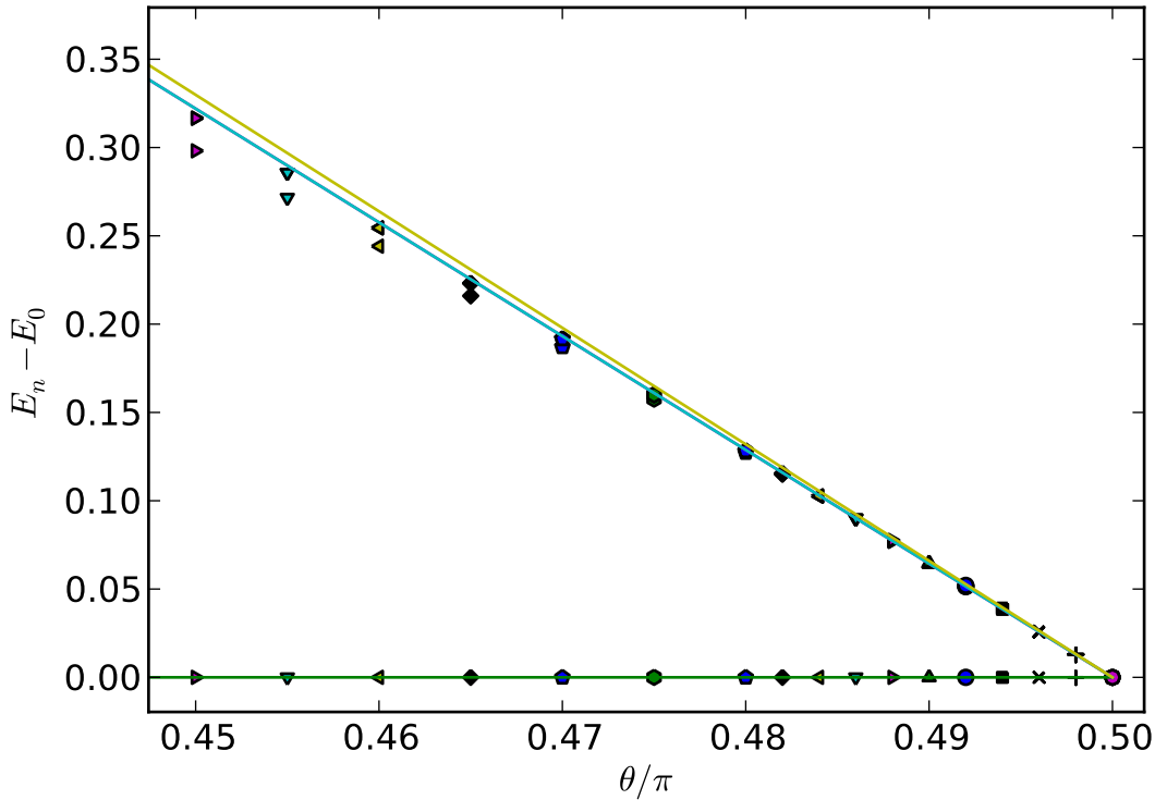
Spectrum of projector model on 6-rung ladder
