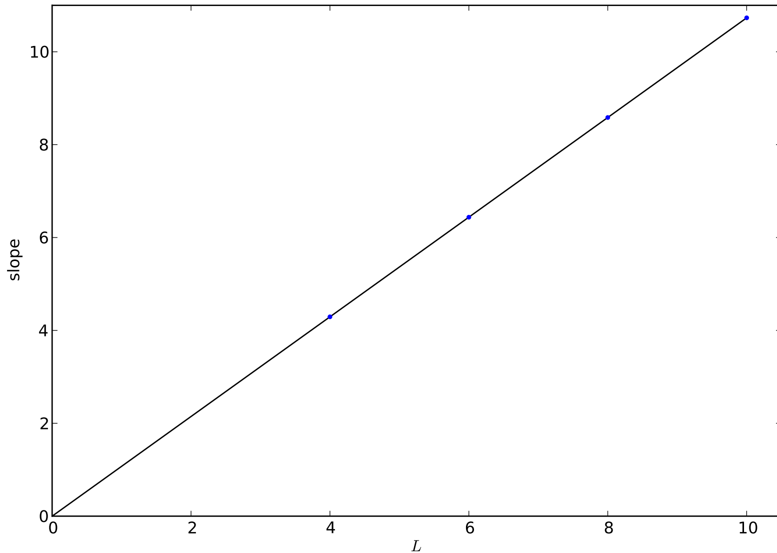
Projector model on ladder: Slope of edge degeneracy lifting
