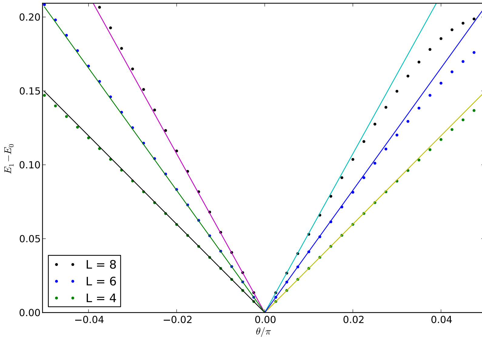
Projector model on ladder: 1st excited state
