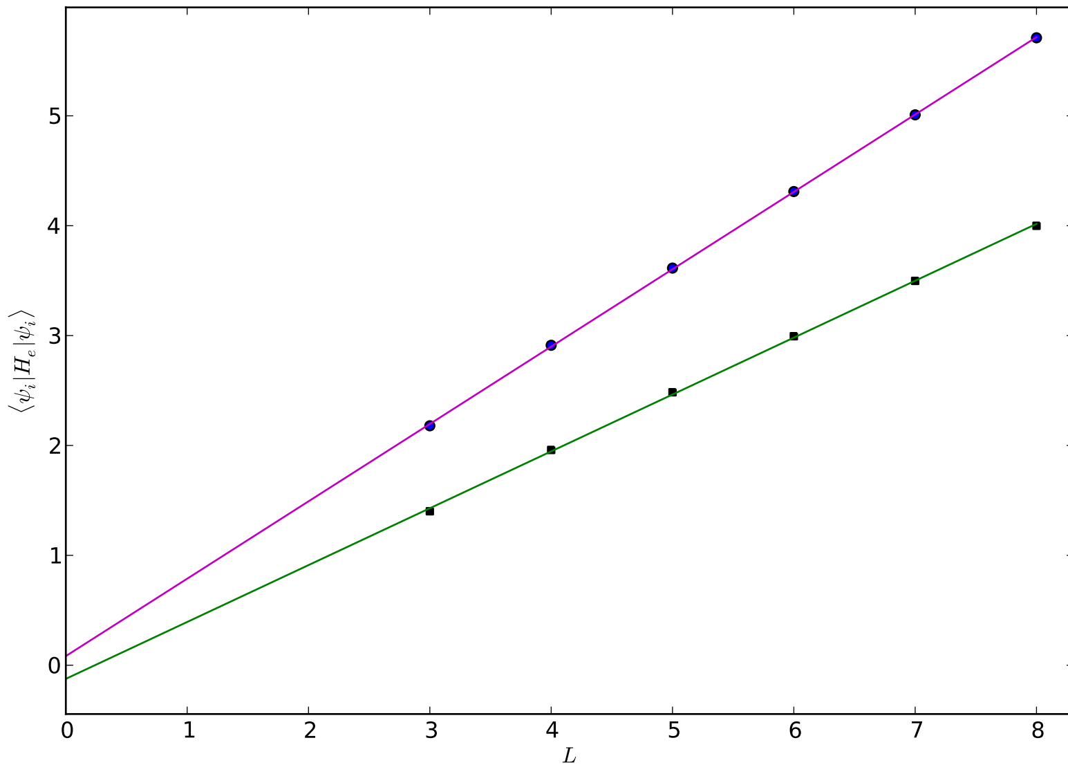
Projector model on ladder: string tension in ground states
