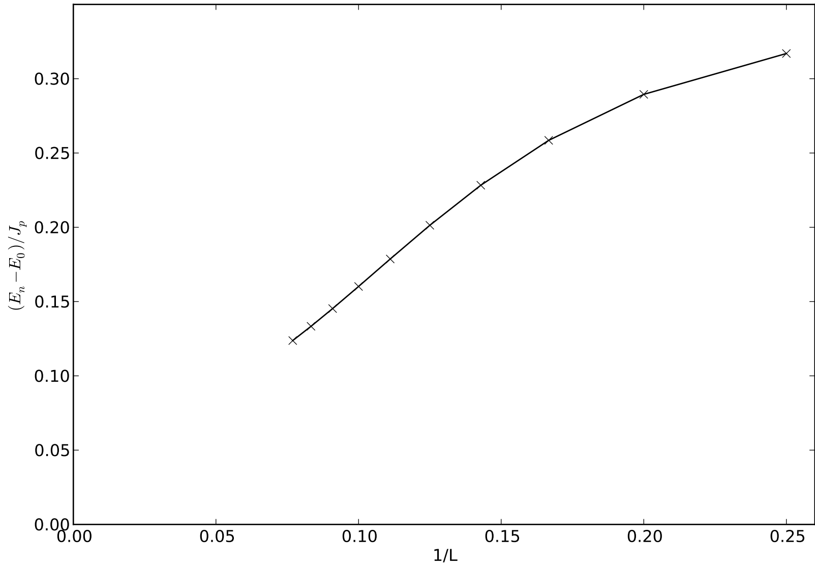
Projector model on ladder \theta=0 : Scaling of the gap
