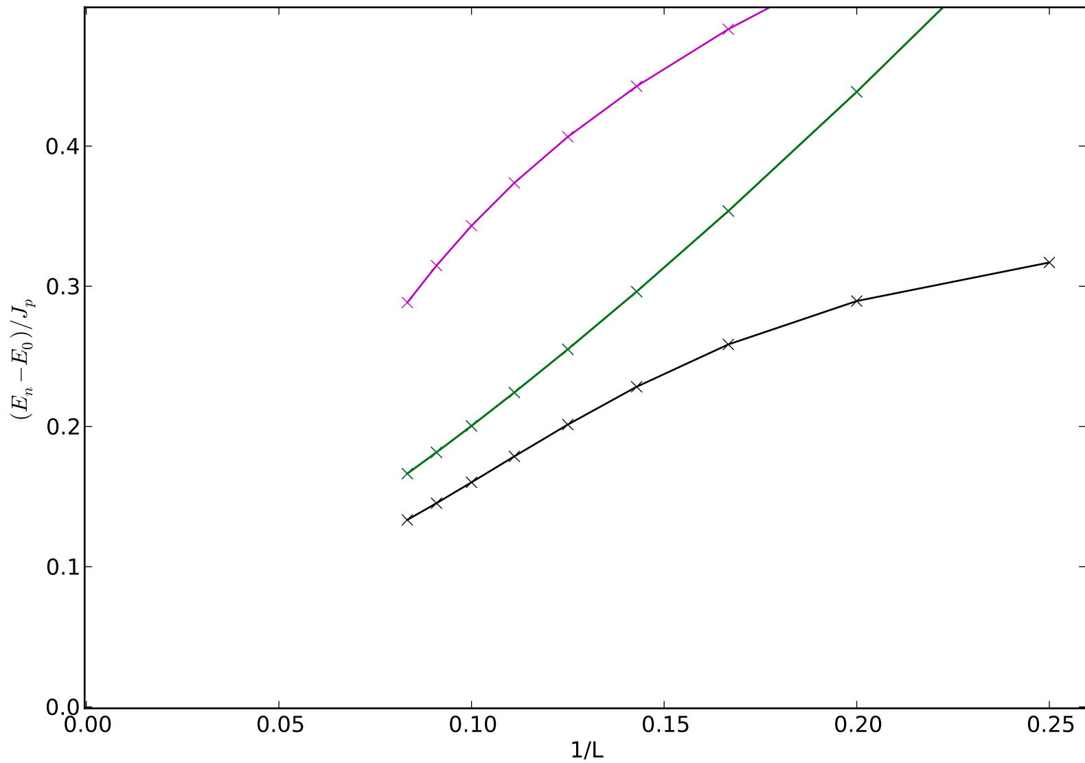
Projector model on ladder \theta=0 : Scaling of lowest states
