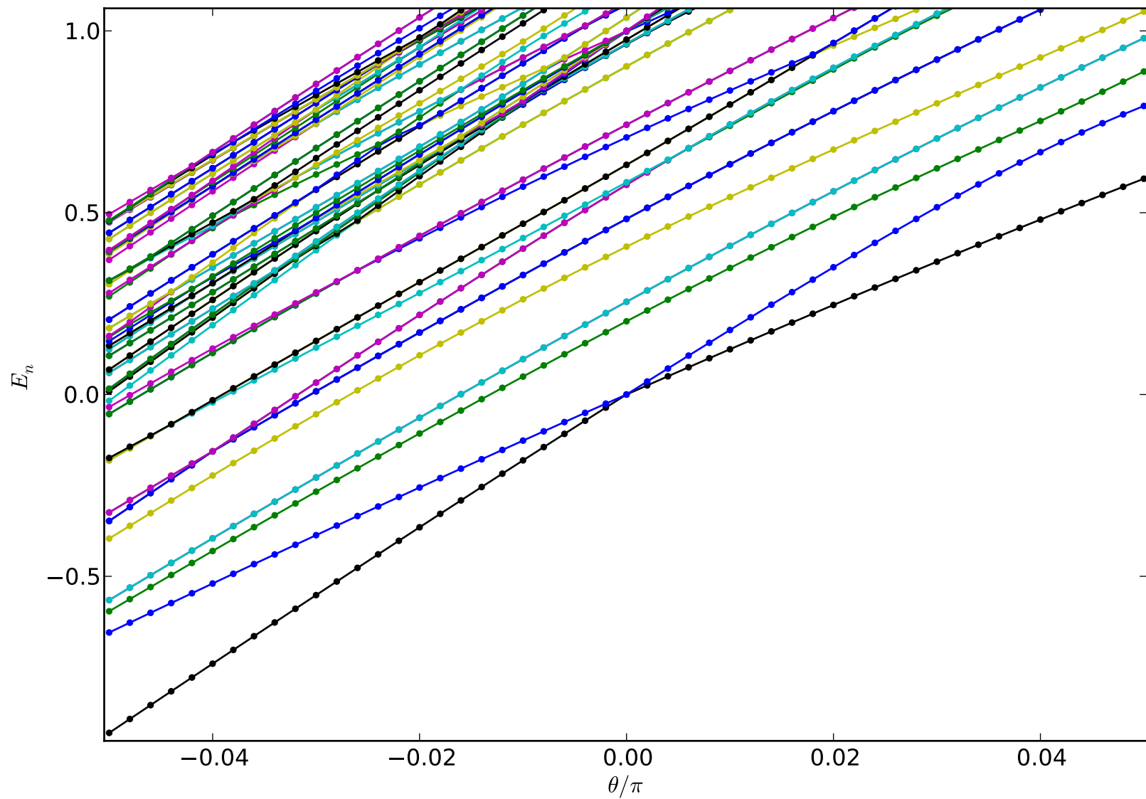
Spectrum of projector model on 8-rung ladder
