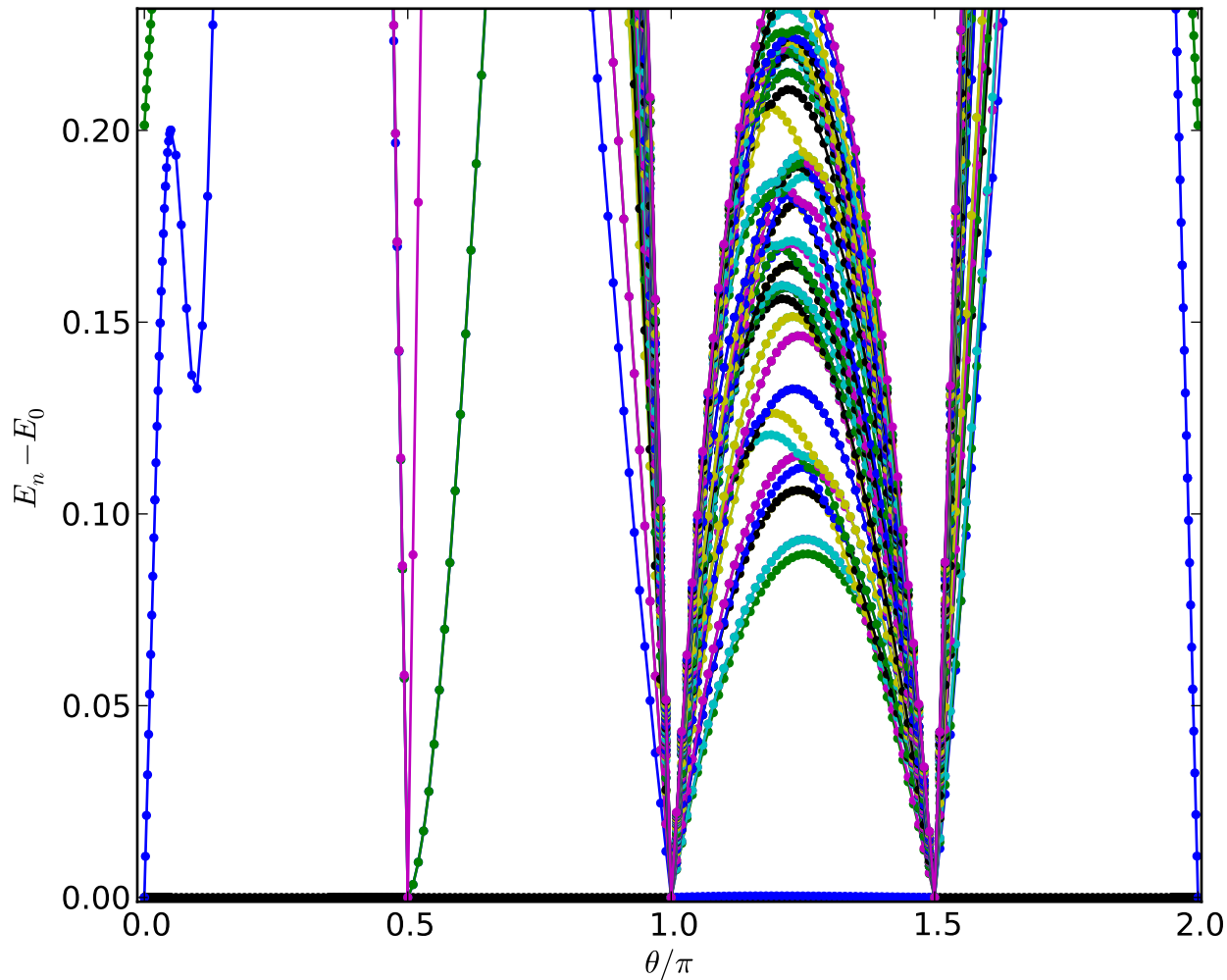
Spectrum of projector model on 8-rung ladder
