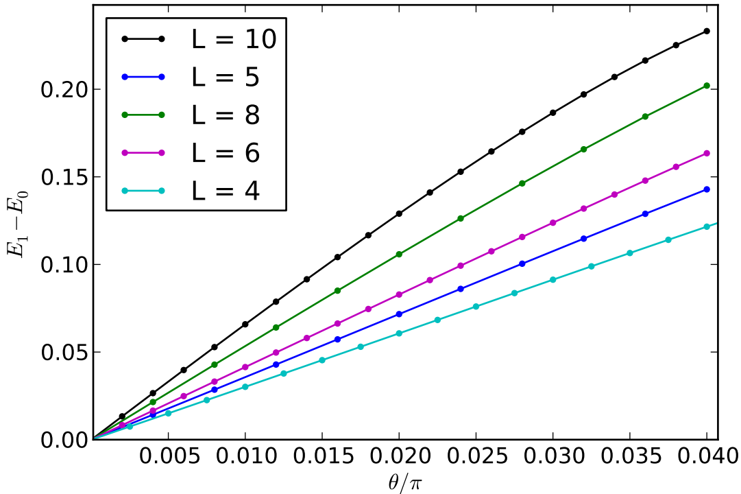
P^\dagger P model on ladder: 1st excited state
