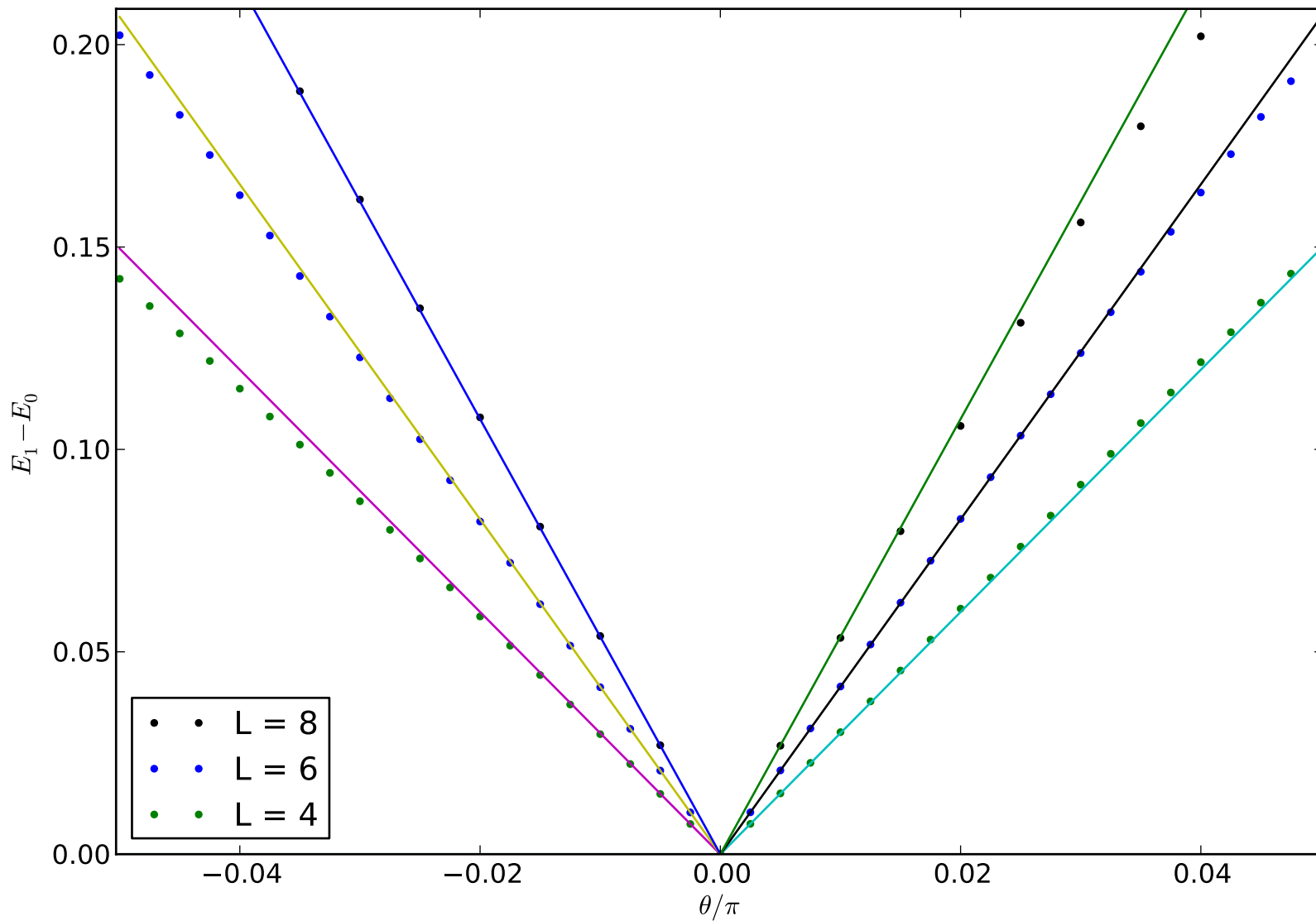
P^\dagger P model on ladder: 1st excited state
