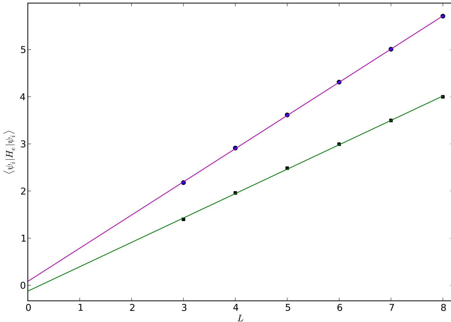
P^\dagger P model on ladder: string tension in ground states
