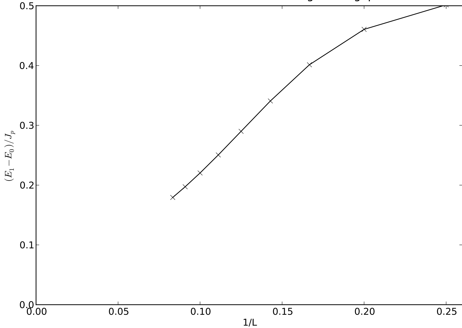
P^\dagger P model on ladder \theta=0 : Scaling of the gap
