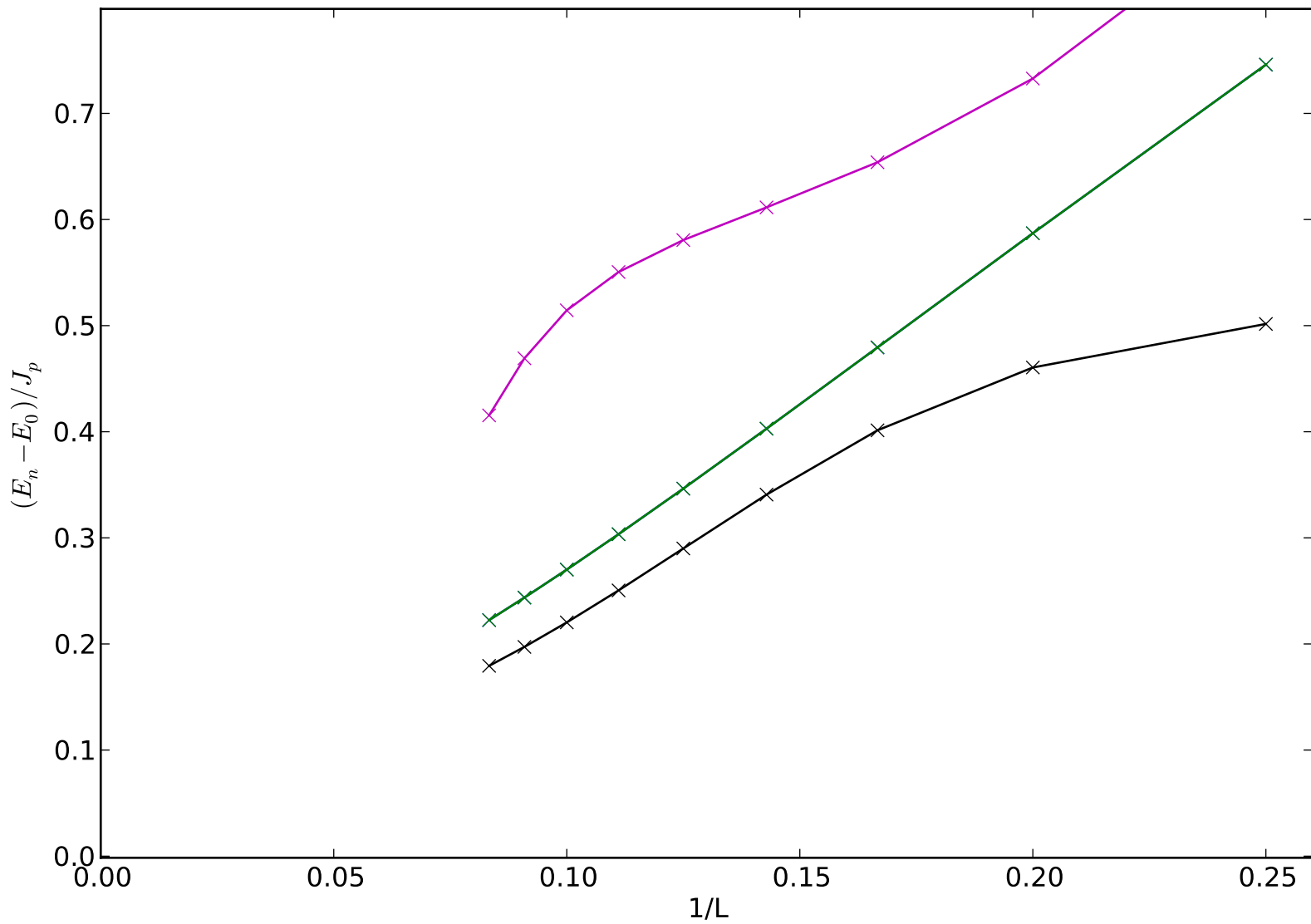
P^\dagger P model on ladder \theta=0 : Scaling of lowest states
