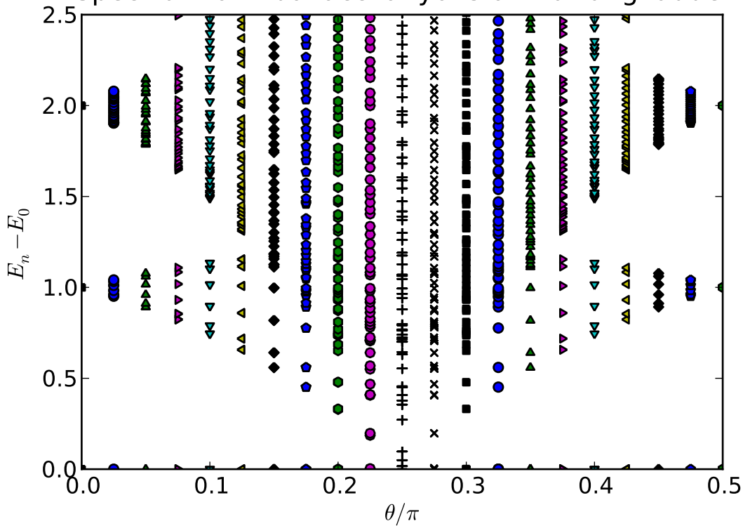
Spectrum of Fibonacci anyons on 10-rung ladder
