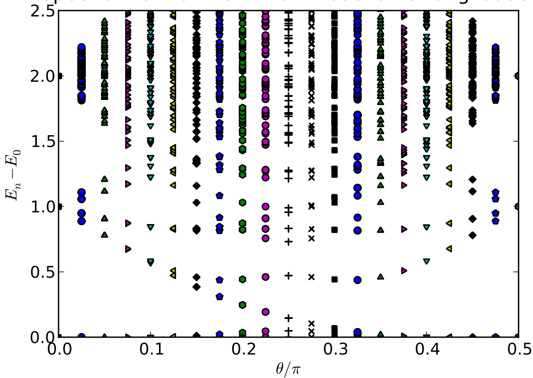
Spectrum of non-hermitian model on 6-rung ladder
