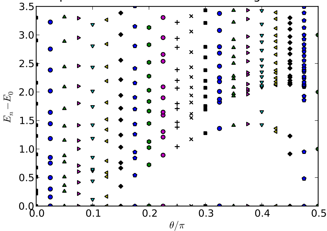
Spectrum of P^\dagger P model on 10-rung ladder
