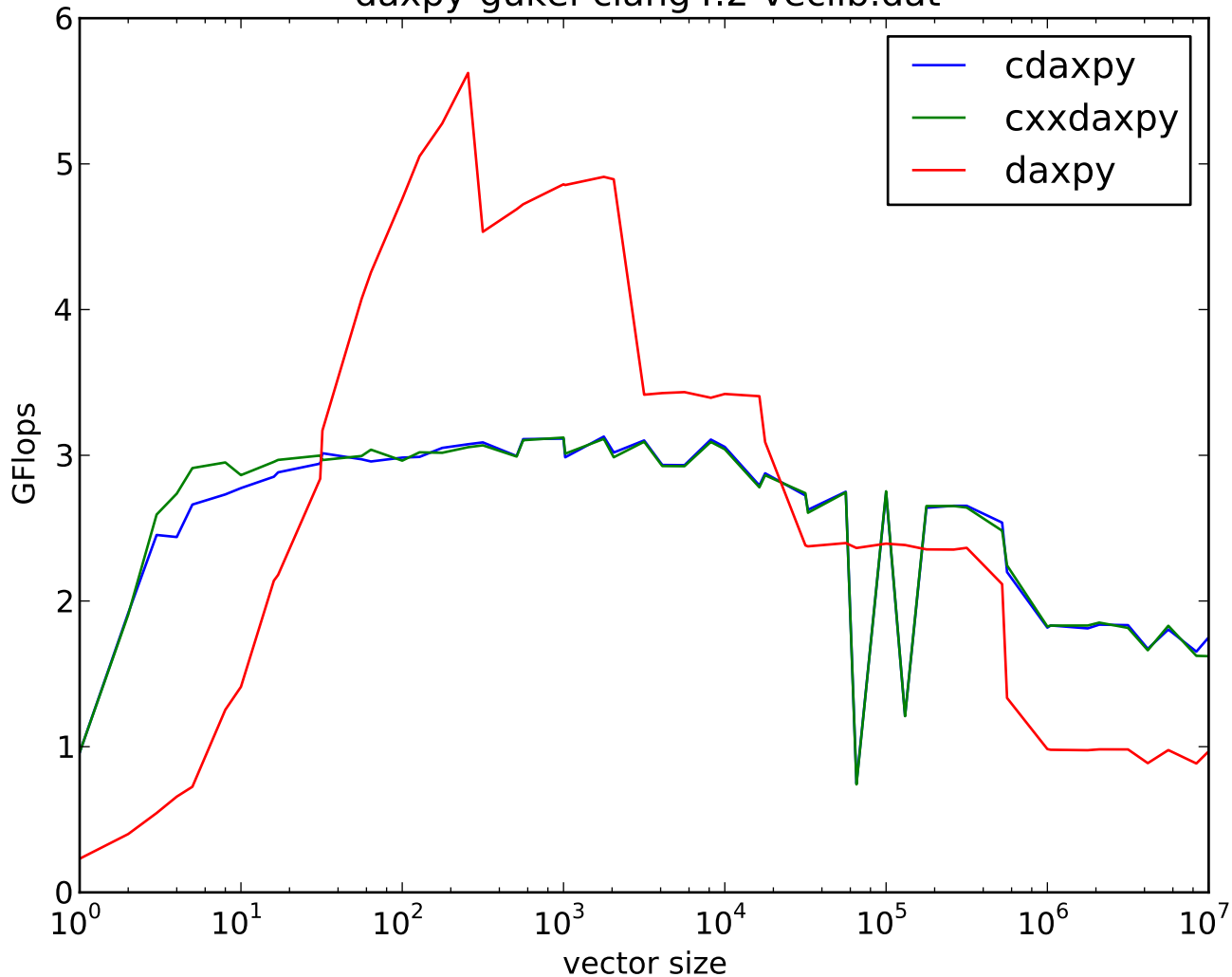
daxpy-gukel-clang4.2-veclib.dat
