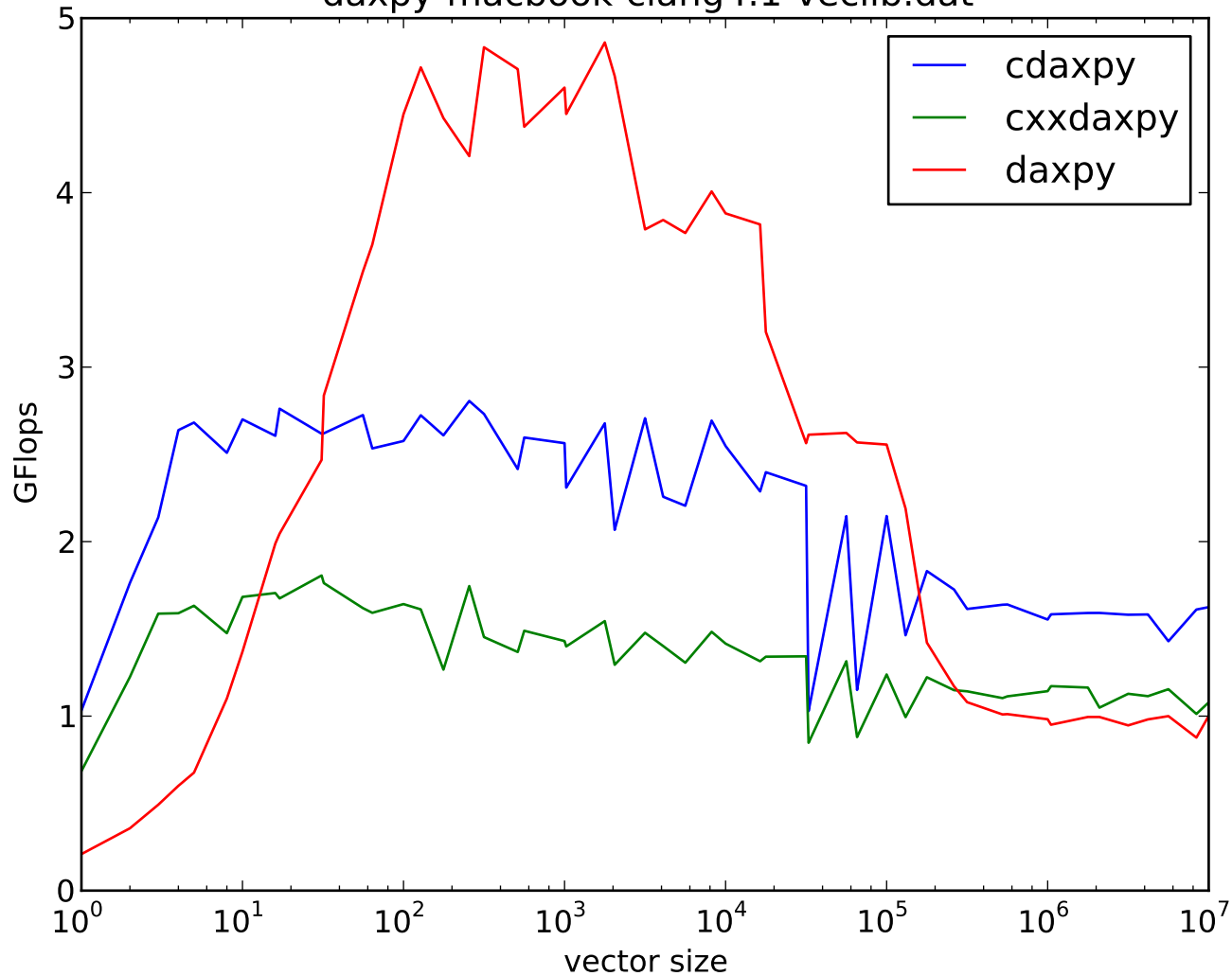
daxpy-macbook-clang4.1-veclib.dat
