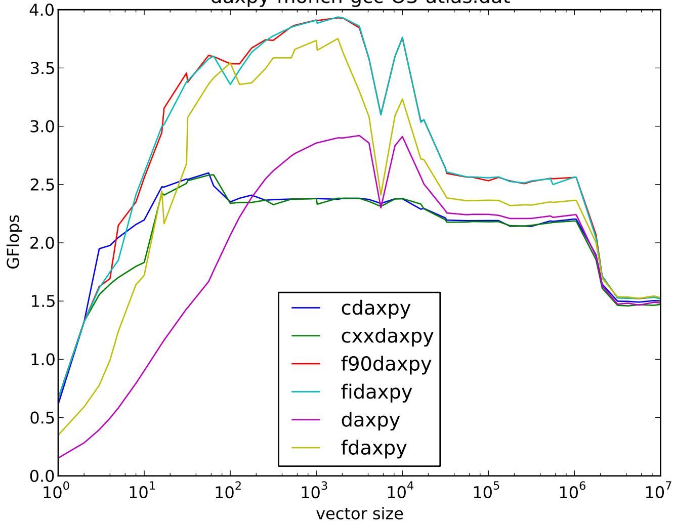
daxpy-monch-gcc-O3-atlas.dat
