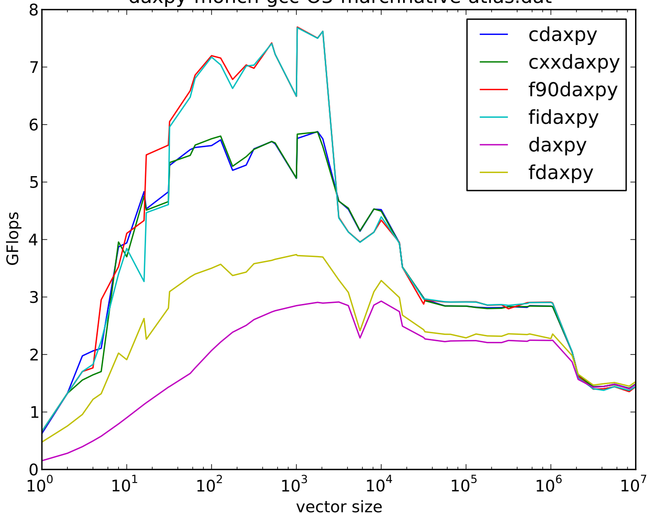
daxpy-monch-gcc-O3-marchnative-atlas.dat
