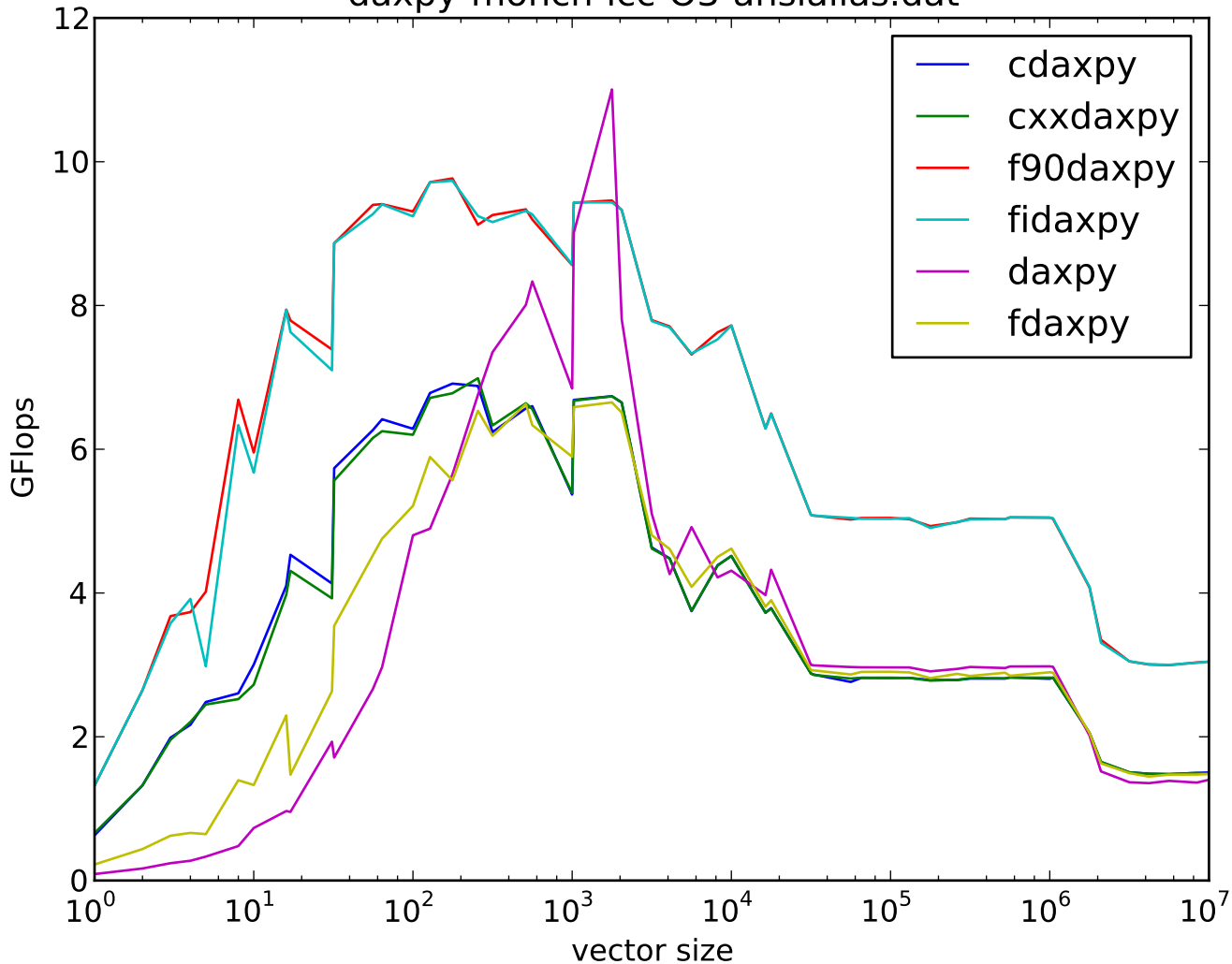
daxpy-monch-icc-O3-ansialias.dat
