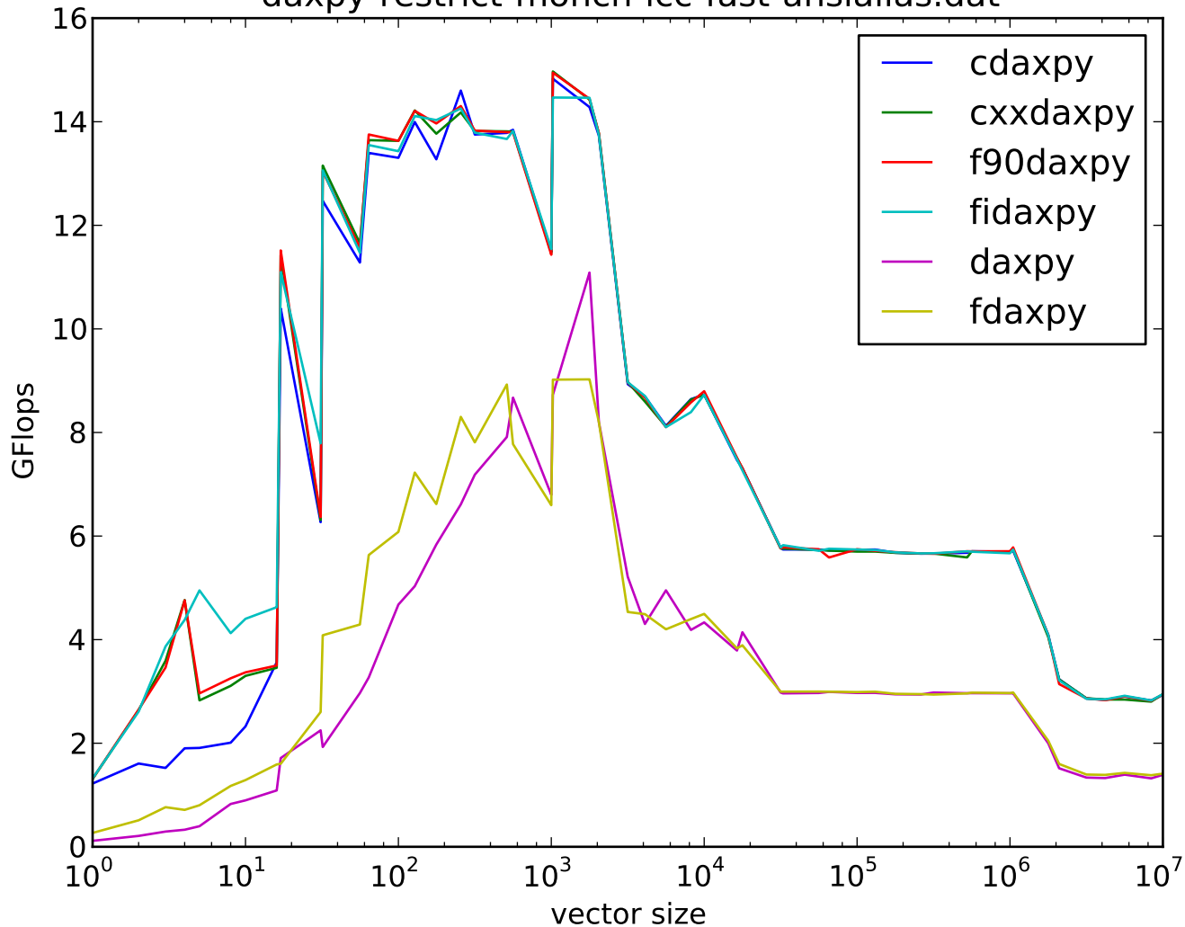
daxpy-restrict-monch-icc-fast-ansialias.dat
