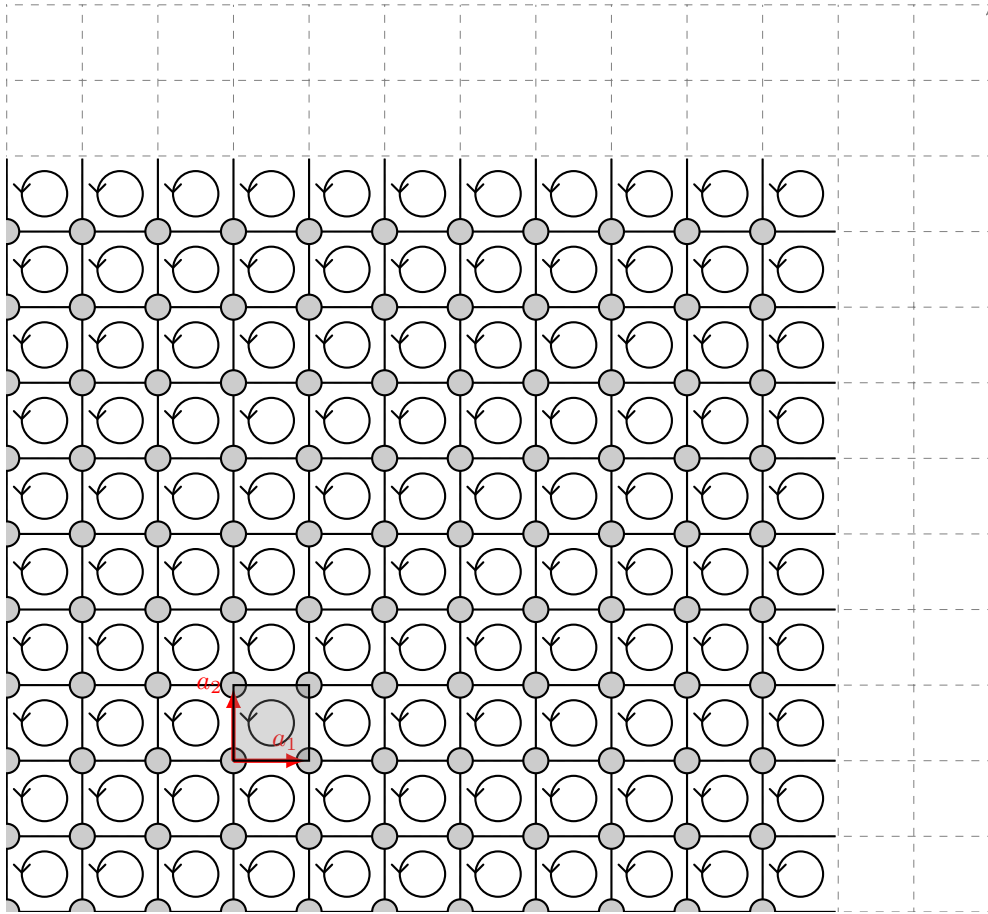
Figure 1: Honeycomb lattice
